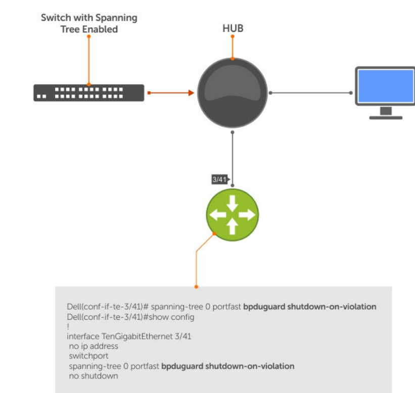
Figure 113. Enabling BPDUGuard
